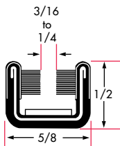
8A1 Flexible Pile Lining Rubber-Covered
