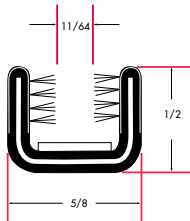
8A8R Rigid Pile Lining Rubber-Covered
